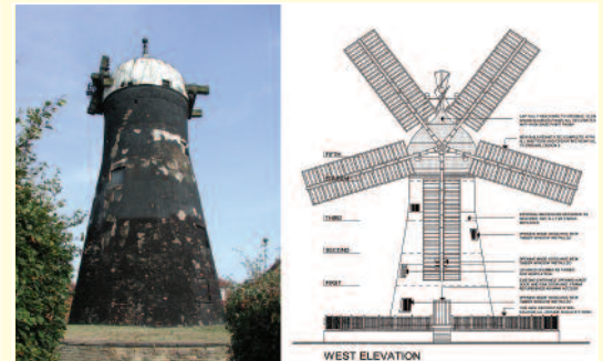
Restoration to full working order of the oldest multi sailed brick tower mill in the UK.
